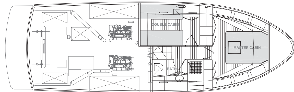
lower deck
